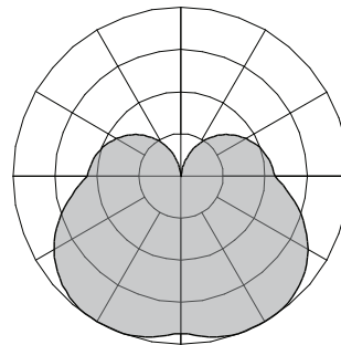
DR - Drop Lens (1-7/8\"/>
