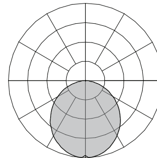
LU - Light Up Lens (1/4\"/>
